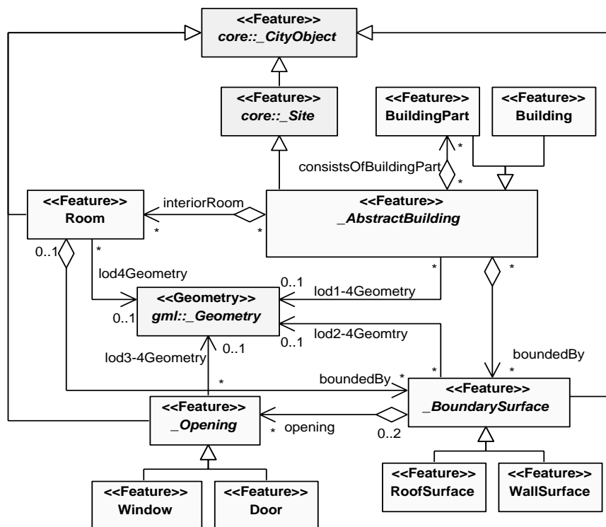
Fig. 5. UML diagram showing a simplified excerpt from the CityGML building model. Attributes are omitted for readability. Please note, that feature classes have multiple relations to geometry classes (e.g. lod1Geometry , lod2Geometry etc.).
