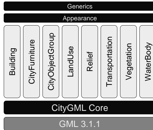
Fig. 2. Modularization of CityGML 1.0.0. Vertical modules contain the semantic modelling for different thematic areas.
