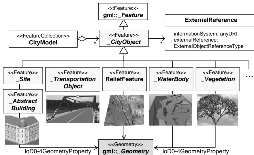
Fig. 4. UML diagram [11] of the top level class hierarchy of CityGML. All thematic objects are considered geographic features (following [10]) and their classes are derived from the abstract superclass CityObject . Attributes are omitted here for readability.
