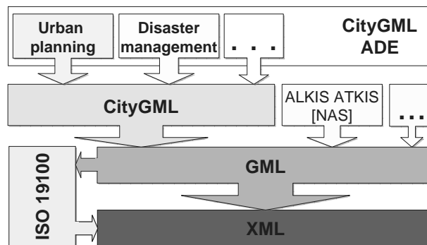
Fig. 7. CityGML Application Domain Extensions are XML schema definitions based on the CityGML schema. They extend CityGML by new feature classes and additional attributes for existing classes. CityGML is an application schema of GML (like others, e.g. the German national cadastre standard ALKIS).
