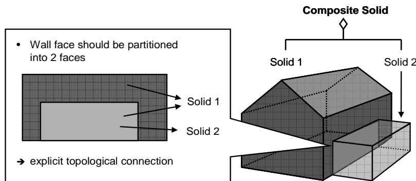
Fig. 6. A building with a connected garage. The topological adjacency between the solids representing the building extent and the garage extent can be made explicit by sharing the common wall surface.
